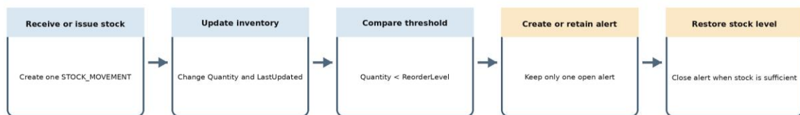
Figure 3 Inventory update and restock alert evaluation flow
